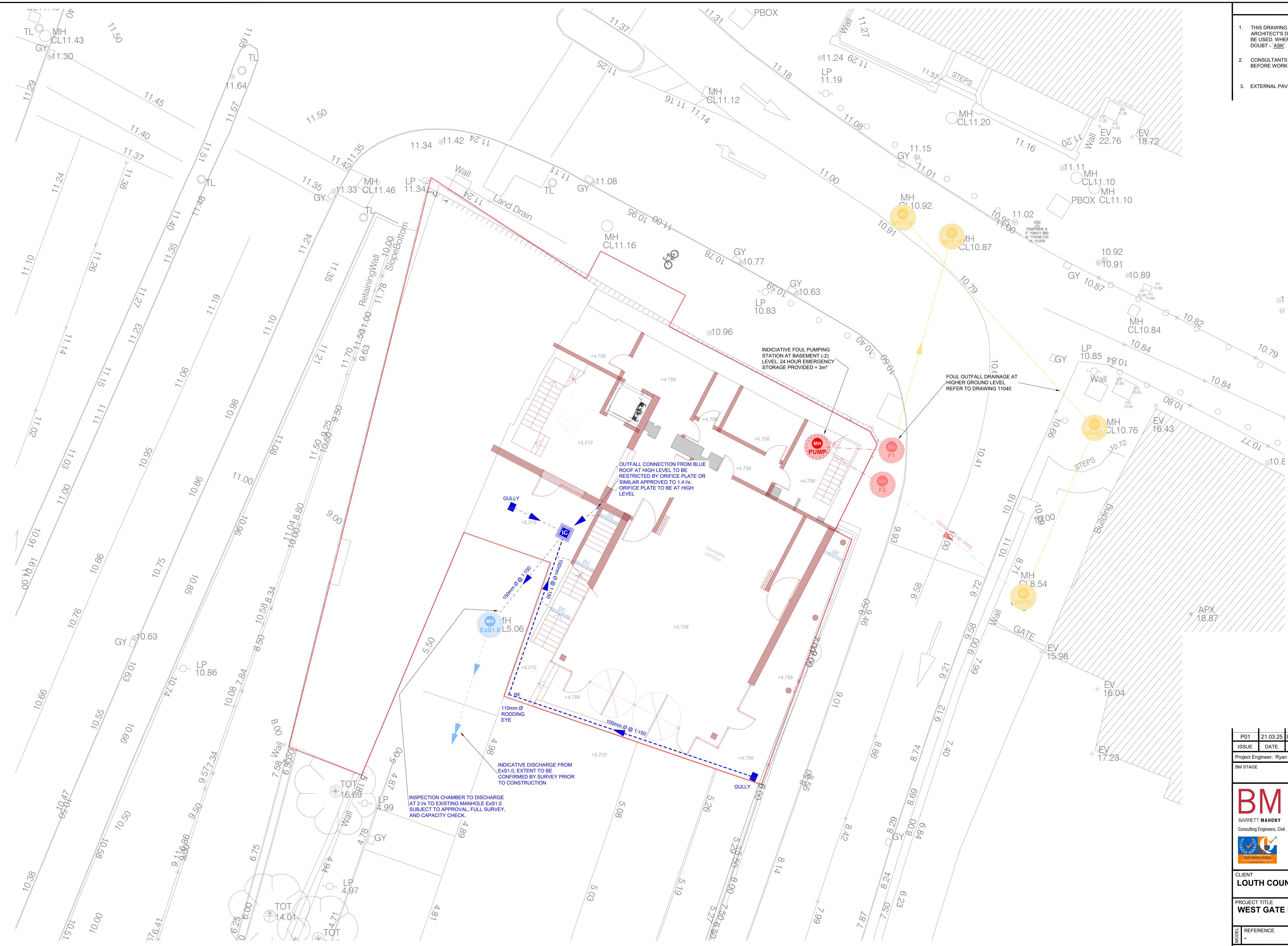
PLAN BASEMENT (-2) FLOOR LEVEL - DRAINAGE LAYOUT
