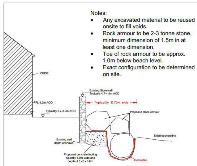
Plate 13. Extract of civil engineering drawings for proposed Coastal Works at Drummullagh showing section through proposed rock armour with concrete footing
